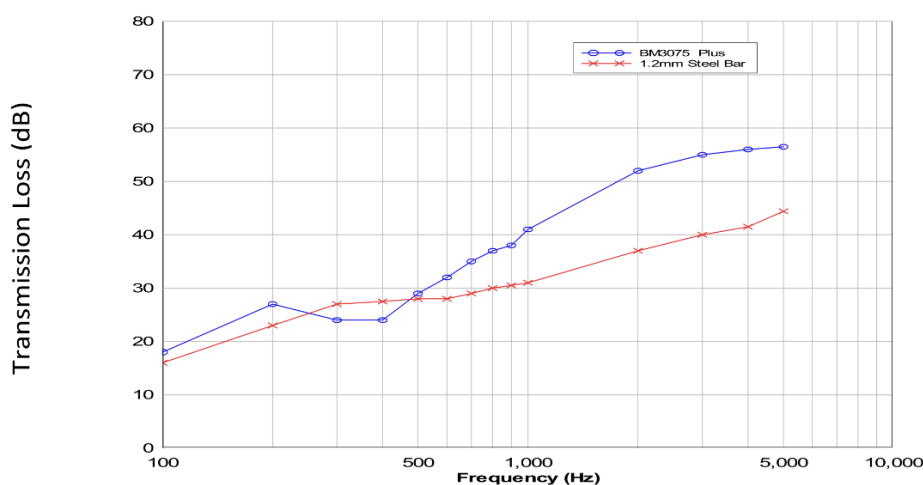
Transmission Loss ESO R140 on Steel plate
